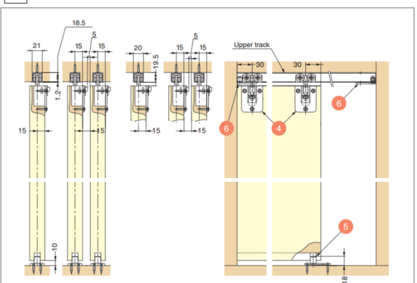
d GFD30 / Side Mount Roller / Standard Sliding
