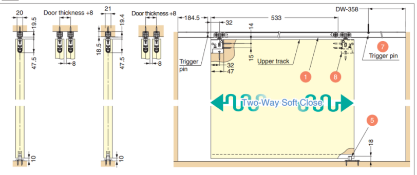
a GFD30 / Recessed Mount Roller / Two-Way Soft Close
