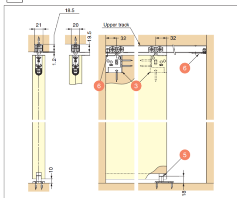
c GFD30 / Recessed Mount Roller / Standard Sliding
