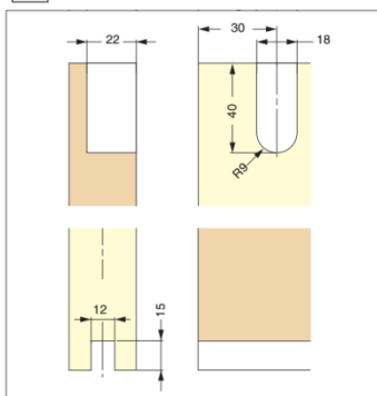
c GFD30 / Recessed Mount Roller / Standard Sliding
